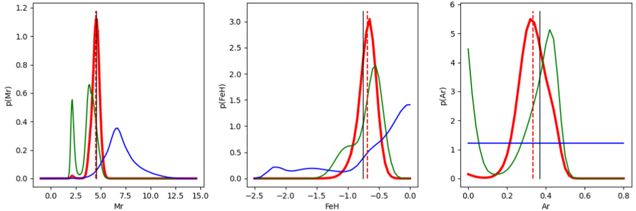
Figure 10. from Lovro Palaversa et al 2025 Astron. J. 169 doi:10.3847/1538-3881/ada3c2 https://dx.doi.org/10.3847/1538-3881/ada3c2 © 2025. The Author(s). Published by the American Astronomical Society.
