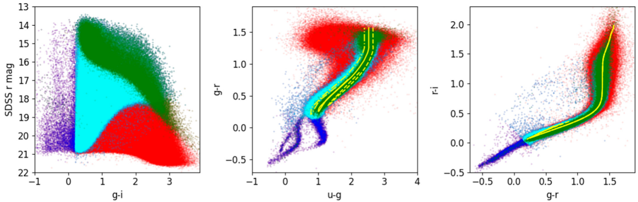
Figure 1. from Lovro Palaversa et al 2025 Astron. J. 169 doi:10.3847/1538-3881/ada3c2 https://dx.doi.org/10.3847/1538-3881/ada3c2 © 2025. The Author(s). Published by the American Astronomical Society.
