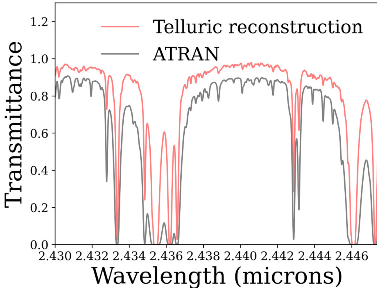
Figure 4. from Arjun B. Savel et al 2025 Astron. J. 169 doi:10.3847/1538-3881/ada27e https://dx.doi.org/10.3847/1538-3881/ada27e © 2025. The Author(s). Published by the American Astronomical Society.
