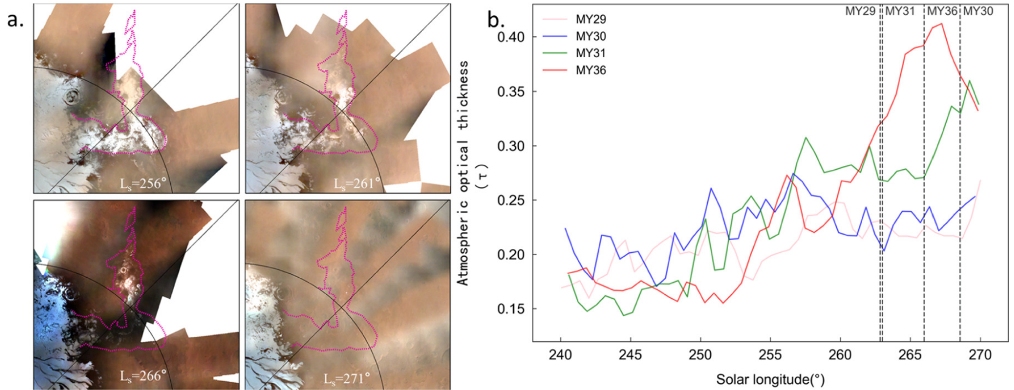
Figure 5. from Zhibin Li et al 2025 Astron. J. 169 doi:10.3847/1538-3881/ada26c https://dx.doi.org/10.3847/1538-3881/ada26c © 2025. The Author(s). Published by the American Astronomical Society.
