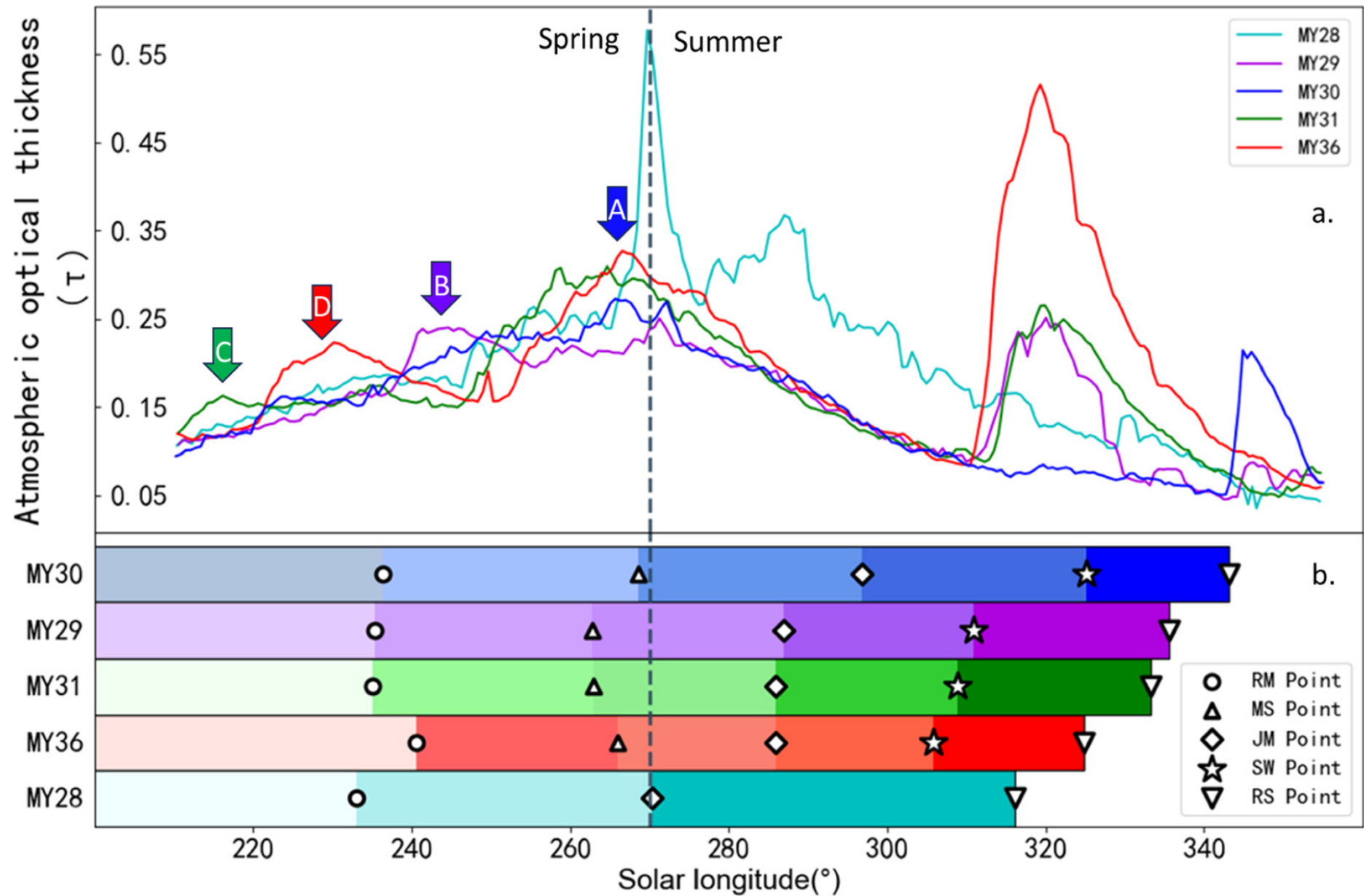
Figure 3. from Zhibin Li et al 2025 Astron. J. 169 doi:10.3847/1538-3881/ada26c https://dx.doi.org/10.3847/1538-3881/ada26c © 2025. The Author(s). Published by the American Astronomical Society.
