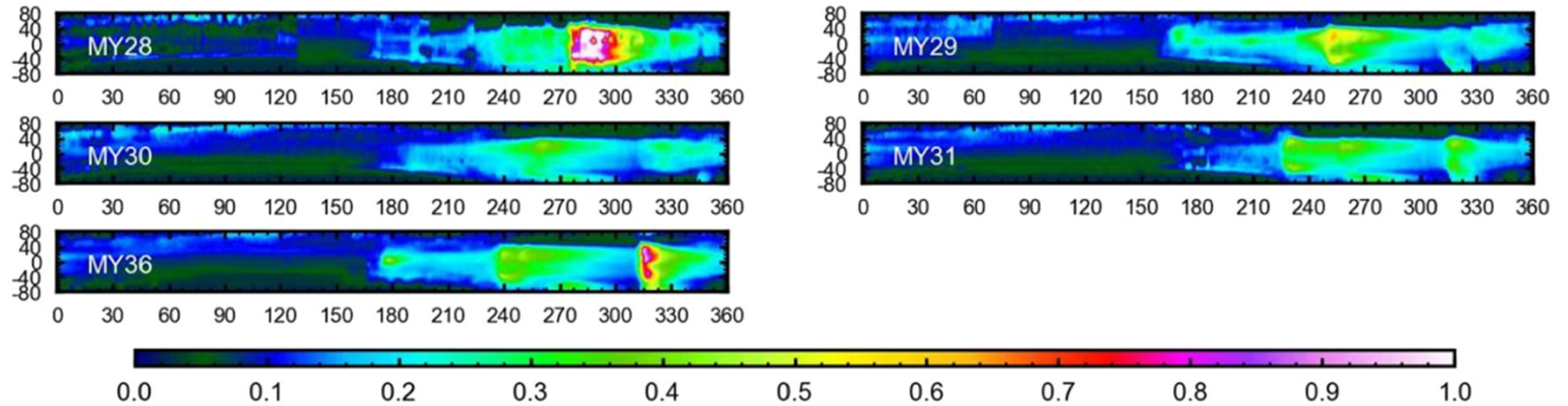
Figure 2. from Zhibin Li et al 2025 Astron. J. 169 doi:10.3847/1538-3881/ada26c https://dx.doi.org/10.3847/1538-3881/ada26c © 2025. The Author(s). Published by the American Astronomical Society.
