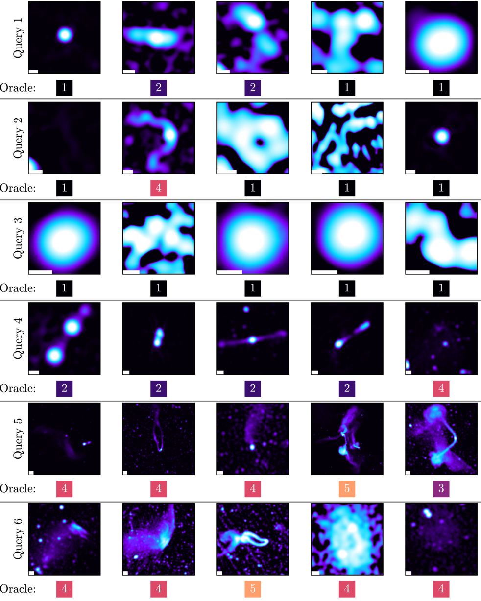
Figure 9. from Michelle Lochner and Lawrence Rudnick 2025 Astron. J. 169 doi:10.3847/1538-3881/ada14c https://dx.doi.org/10.3847/1538-3881/ada14c © 2025. The Author(s). Published by the American Astronomical Society.
