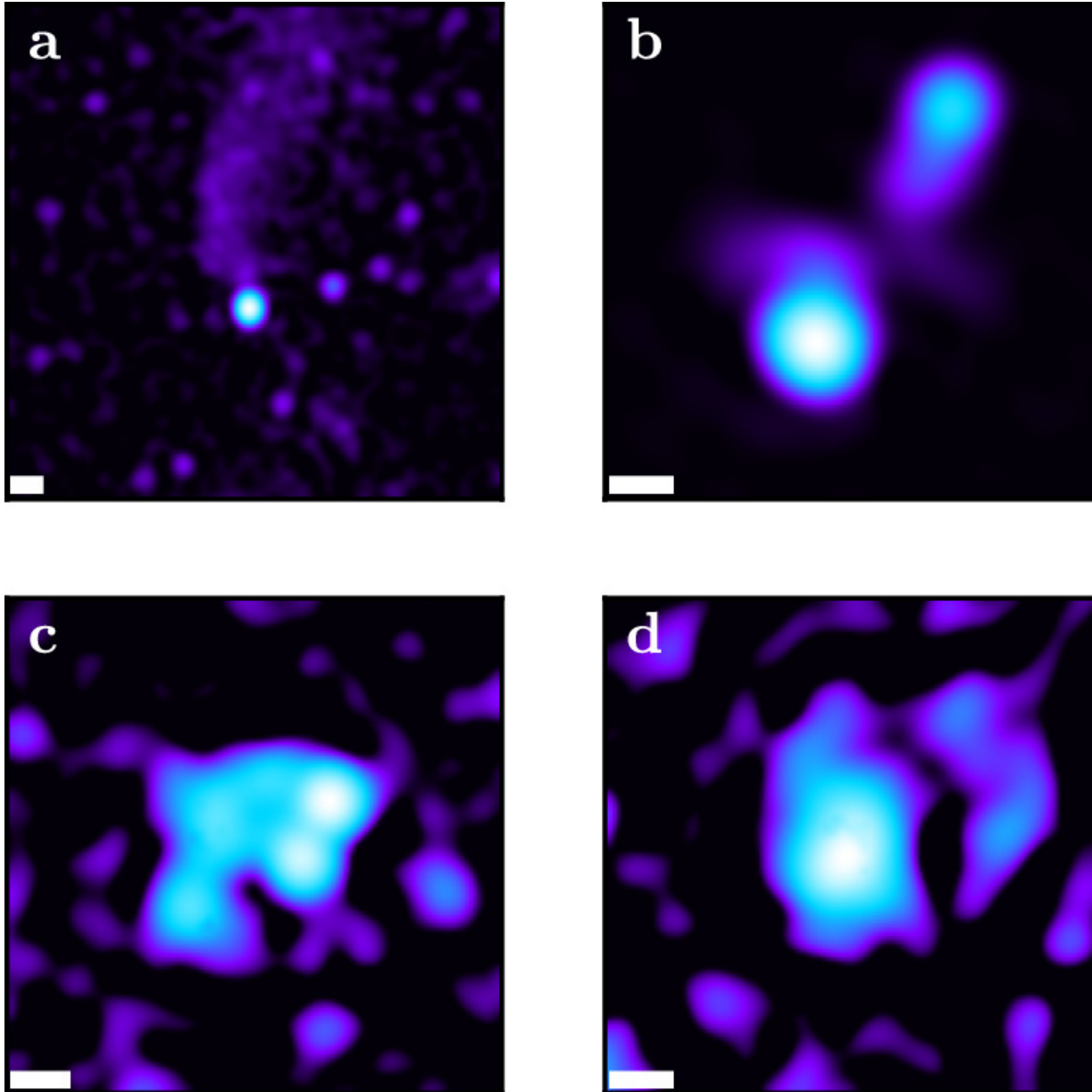
Figure 7. from Michelle Lochner and Lawrence Rudnick 2025 Astron. J. 169 doi:10.3847/1538-3881/ada14c https://dx.doi.org/10.3847/1538-3881/ada14c © 2025. The Author(s). Published by the American Astronomical Society.
