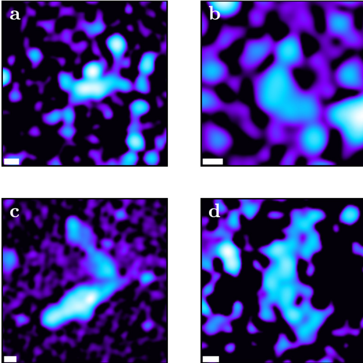
Figure 6. from Michelle Lochner and Lawrence Rudnick 2025 Astron. J. 169 doi:10.3847/1538-3881/ada14c https://dx.doi.org/10.3847/1538-3881/ada14c © 2025. The Author(s). Published by the American Astronomical Society.
