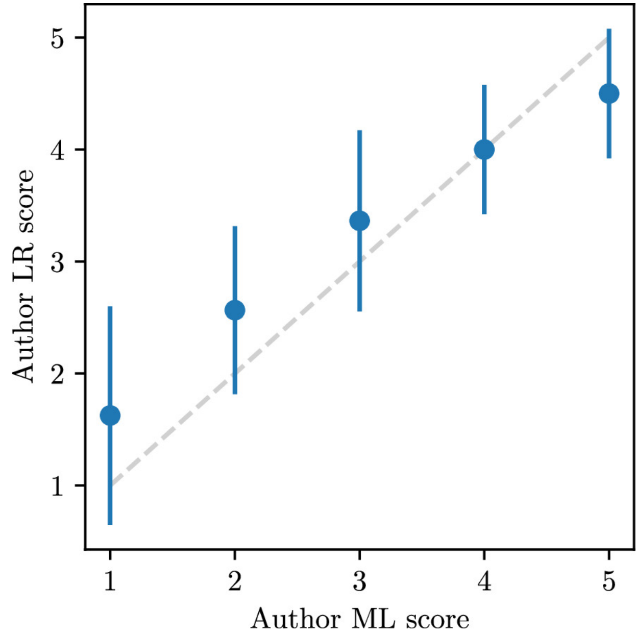
Figure 5. from Michelle Lochner and Lawrence Rudnick 2025 Astron. J. 169 doi:10.3847/1538-3881/ada14c https://dx.doi.org/10.3847/1538-3881/ada14c © 2025. The Author(s). Published by the American Astronomical Society.
