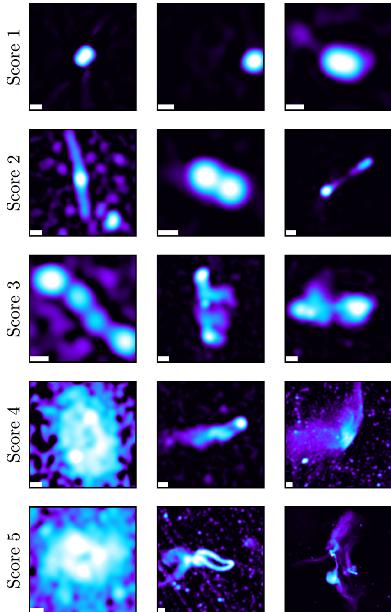
Figure 4. from Michelle Lochner and Lawrence Rudnick 2025 Astron. J. 169 doi:10.3847/1538-3881/ada14c https://dx.doi.org/10.3847/1538-3881/ada14c © 2025. The Author(s). Published by the American Astronomical Society.
