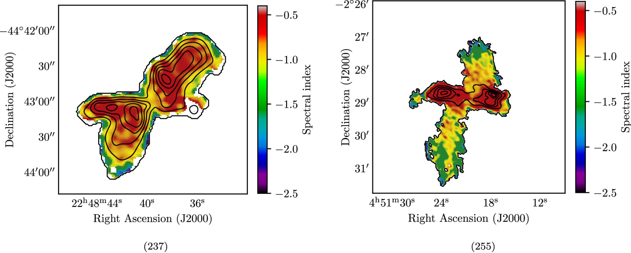
Figure 17. from Michelle Lochner and Lawrence Rudnick 2025 Astron. J. 169 doi:10.3847/1538-3881/ada14c https://dx.doi.org/10.3847/1538-3881/ada14c © 2025. The Author(s). Published by the American Astronomical Society.
