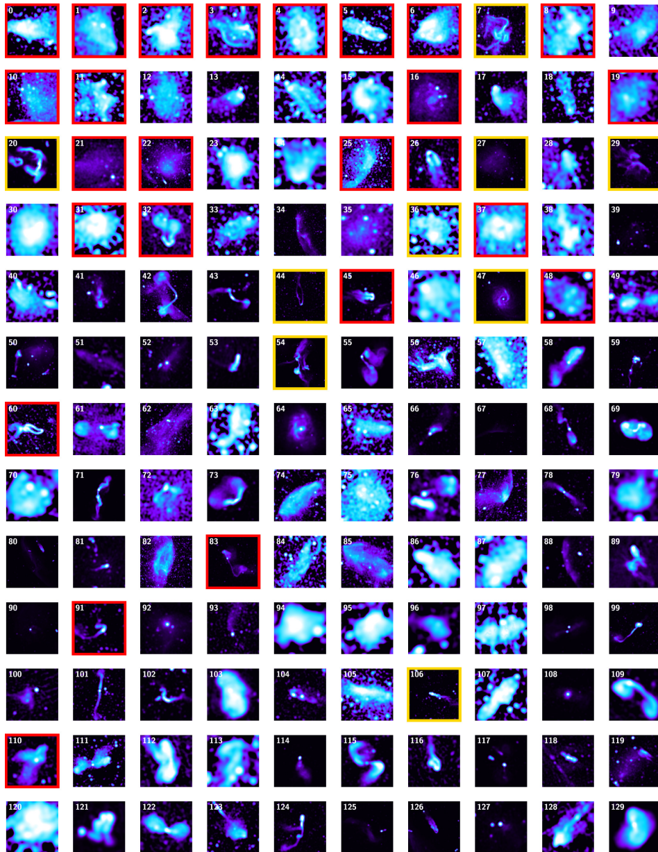
Figure 15. from Michelle Lochner and Lawrence Rudnick 2025 Astron. J. 169 doi:10.3847/1538-3881/ada14c https://dx.doi.org/10.3847/1538-3881/ada14c © 2025. The Author(s). Published by the American Astronomical Society.
