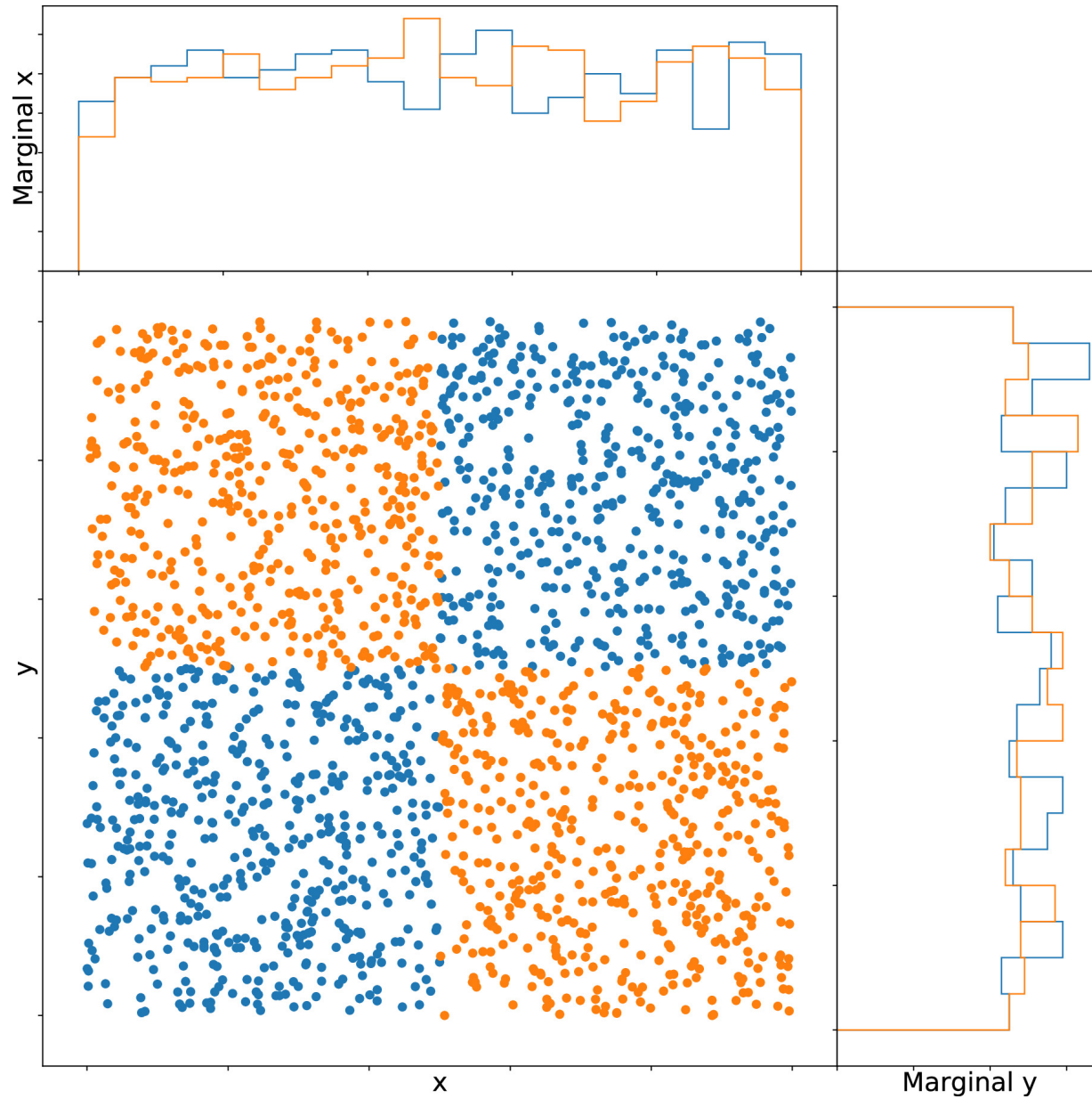
Figure 7. from Jacob A. Kurlander et al 2025 Astron. J. 169 doi:10.3847/1538-3881/ad9a58 https://dx.doi.org/10.3847/1538-3881/ad9a58 © 2025. The Author(s). Published by the American Astronomical Society.
