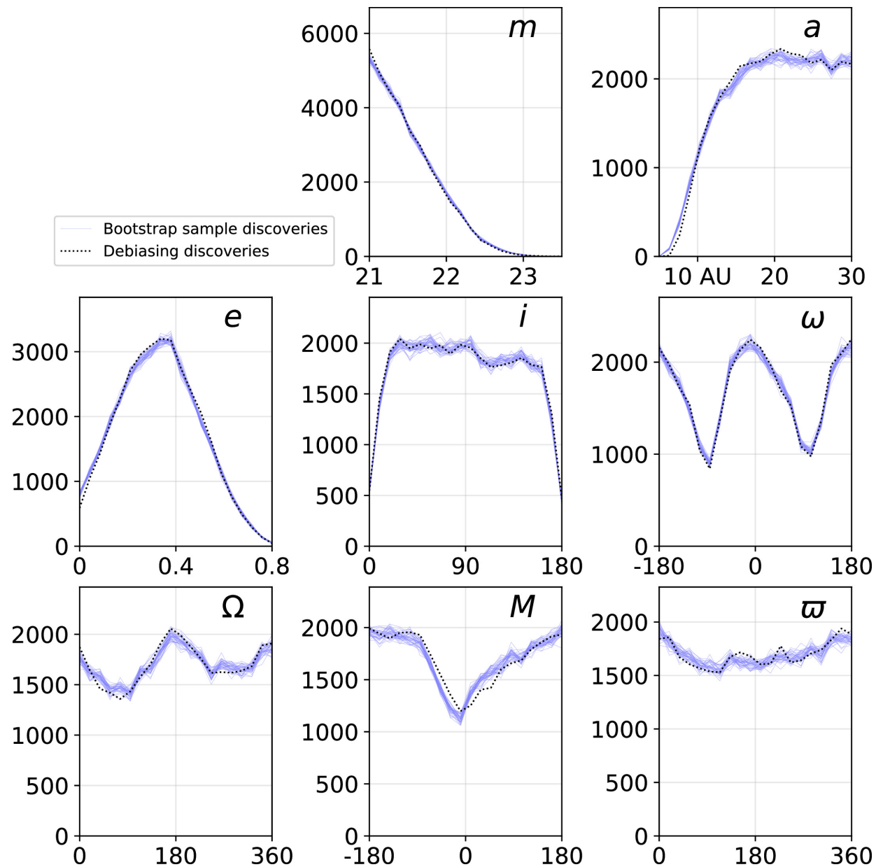
Figure 5. from Jacob A. Kurlander et al 2025 Astron. J. 169 doi:10.3847/1538-3881/ad9a58 https://dx.doi.org/10.3847/1538-3881/ad9a58 © 2025. The Author(s). Published by the American Astronomical Society.
