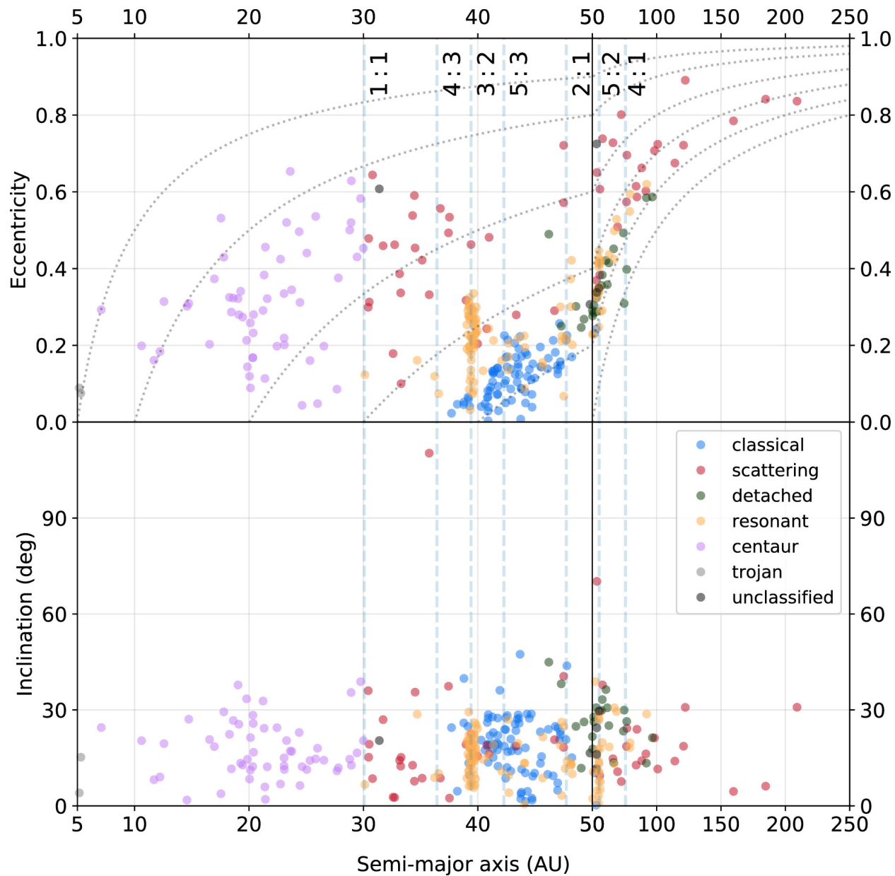
Figure 3. from Jacob A. Kurlander et al 2025 Astron. J. 169 doi:10.3847/1538-3881/ad9a58 https://dx.doi.org/10.3847/1538-3881/ad9a58 © 2025. The Author(s). Published by the American Astronomical Society.
