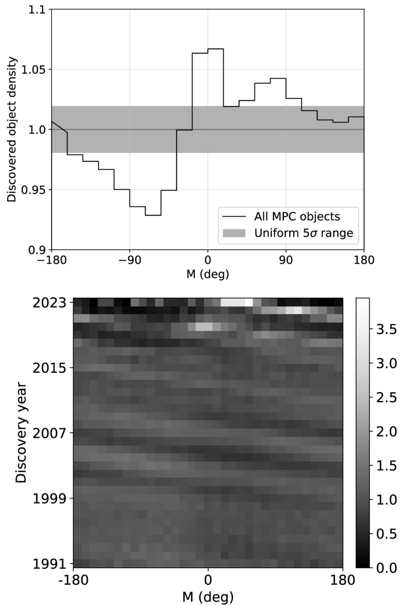
Figure 1. from Jacob A. Kurlander et al 2025 Astron. J. 169 doi:10.3847/1538-3881/ad9a58 https://dx.doi.org/10.3847/1538-3881/ad9a58 © 2025. The Author(s). Published by the American Astronomical Society.
