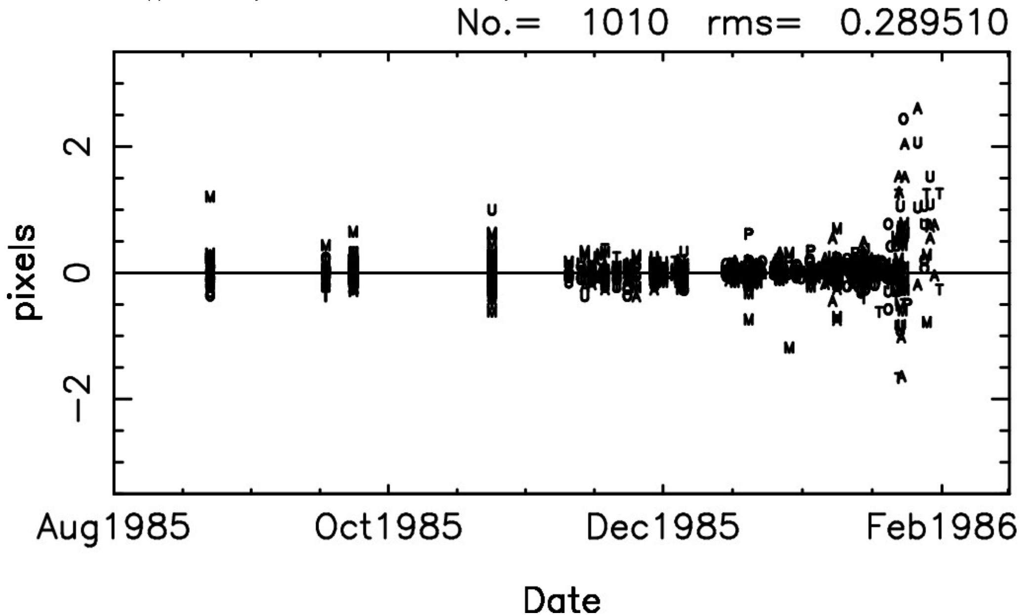
Figure 6. from Robert A. Jacobson and Ryan S. Park 2025 Astron. J. 169 doi:10.3847/1538-3881/ad99d1 https://dx.doi.org/10.3847/1538-3881/ad99d1 © 2025. The Author(s). Published by the American Astronomical Society.
