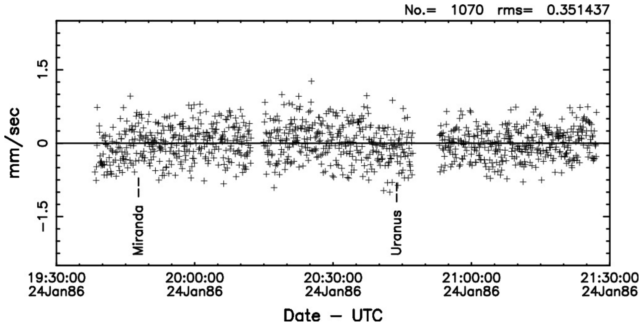
Figure 5. from Robert A. Jacobson and Ryan S. Park 2025 Astron. J. 169 doi:10.3847/1538-3881/ad99d1 https://dx.doi.org/10.3847/1538-3881/ad99d1 © 2025. The Author(s). Published by the American Astronomical Society.
