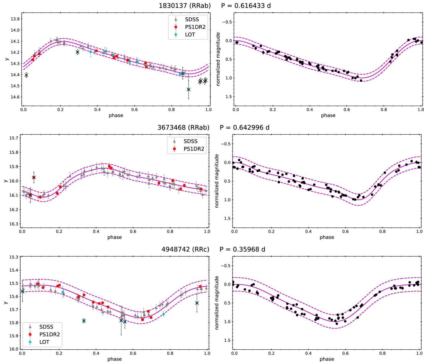
Figure 2. from Chow-Choong Ngeow and Chia-Yu Cheng 2025 Astron. J. 169 doi:10.3847/1538-3881/ad99cf https://dx.doi.org/10.3847/1538-3881/ad99cf © 2025. The Author(s). Published by the American Astronomical Society.
