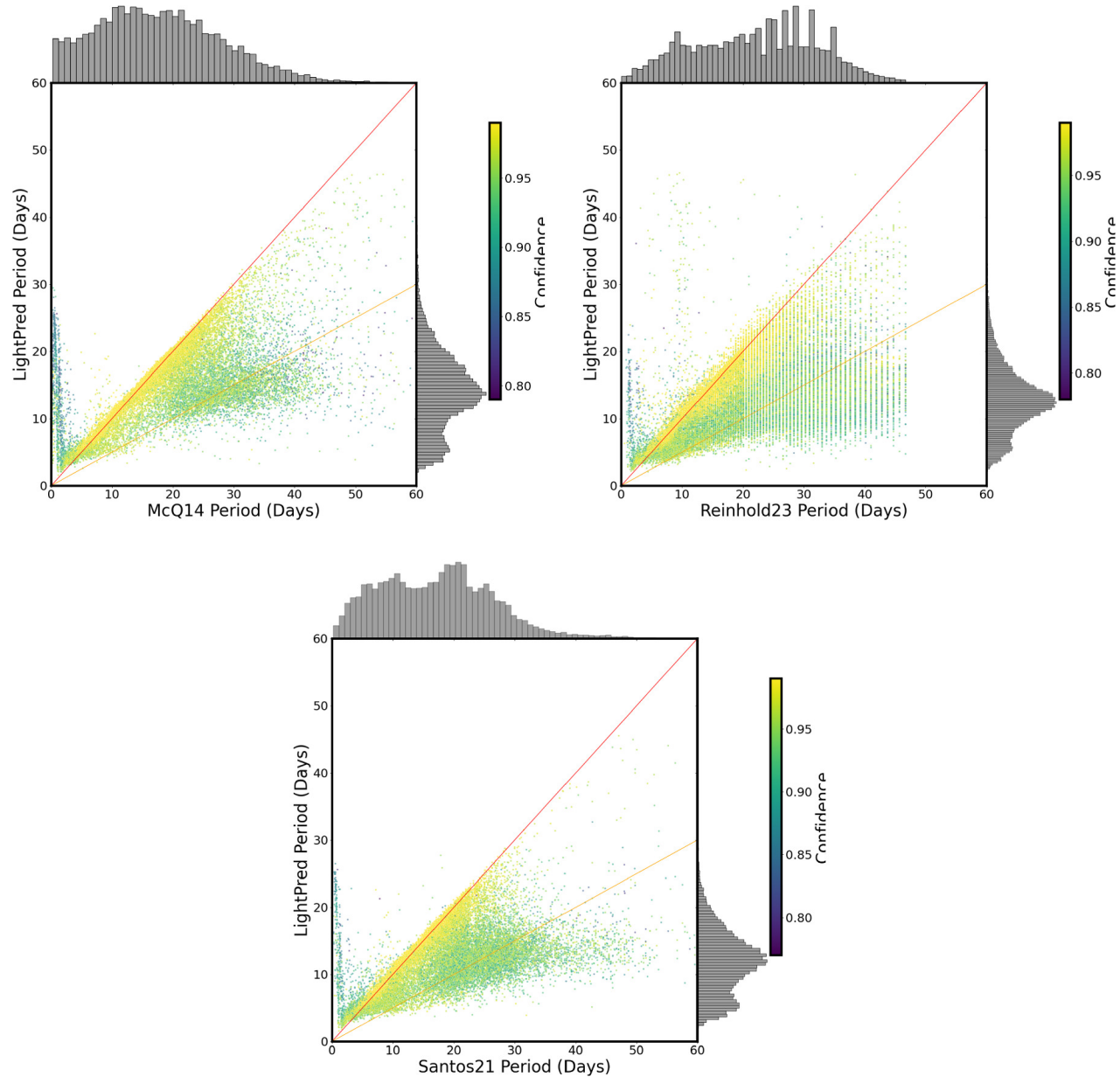
Figure 9. from Ilay Kamai and Hagai B. Perets 2025 Astron. J. 169 doi:10.3847/1538-3881/ad99ab https://dx.doi.org/10.3847/1538-3881/ad99ab © 2025. The Author(s). Published by the American Astronomical Society.
