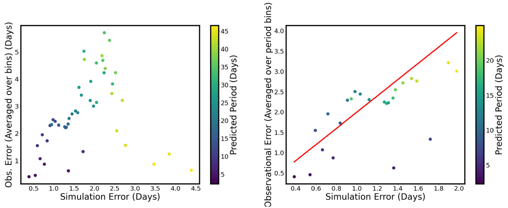
Figure 7. from Illy Kamai and Hagai B. Perets 2025 Astron. J. 169 doi:10.3847/1538-3881/ad99ab https://dx.doi.org/10.3847/1538-3881/ad99ab © 2025. The Author(s). Published by the American Astronomical Society.
