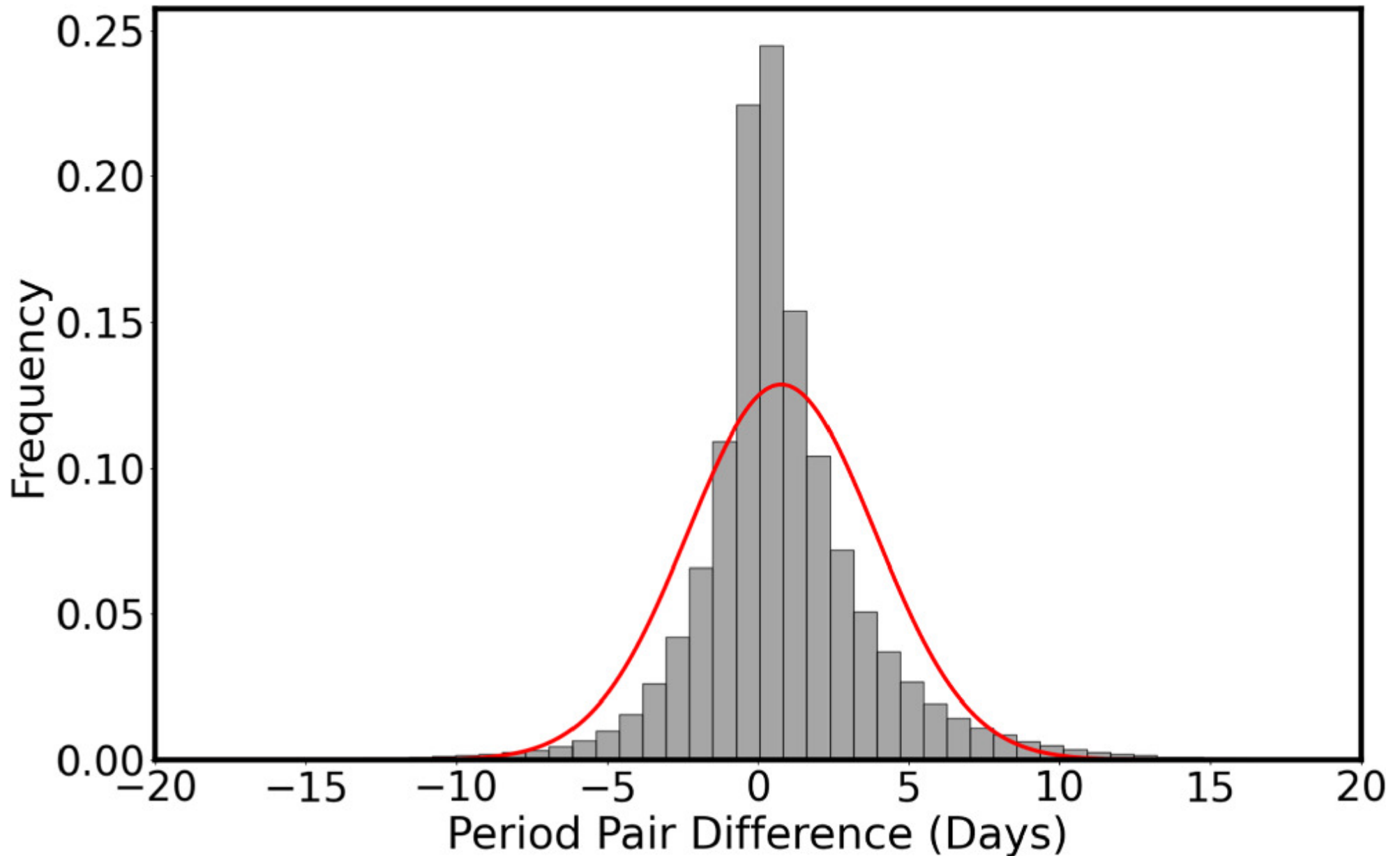
Figure 6. from Ilay Kamai and Hagai B. Perets 2025 Astron. J. 169 doi:10.3847/1538-3881/ad99ab https://dx.doi.org/10.3847/1538-3881/ad99ab © 2025. The Author(s). Published by the American Astronomical Society.
