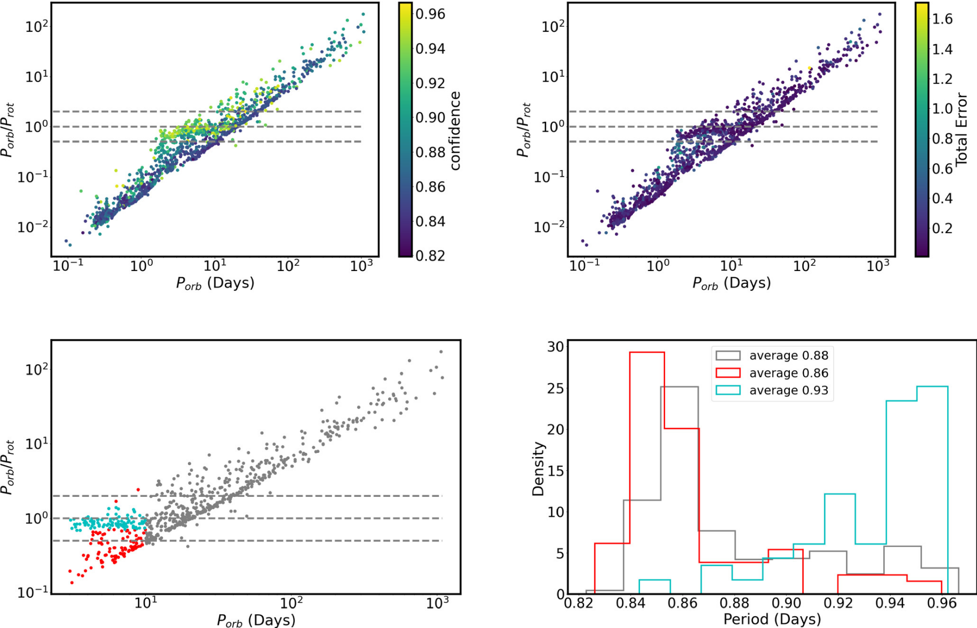
Figure 16. from Ilay Kamai and Hagai B. Perets 2025 Astron. J. 169 doi:10.3847/1538-3881/ad99ab https://dx.doi.org/10.3847/1538-3881/ad99ab © 2025. The Author(s). Published by the American Astronomical Society.
