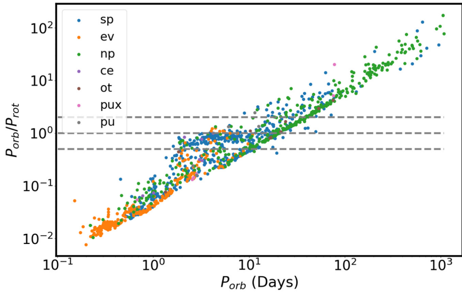
Figure 15. from Ilay Kamai and Hagai B. Perets 2025 Astron. J. 169 doi:10.3847/1538-3881/ad99ab https://dx.doi.org/10.3847/1538-3881/ad99ab © 2025. The Author(s). Published by the American Astronomical Society.
