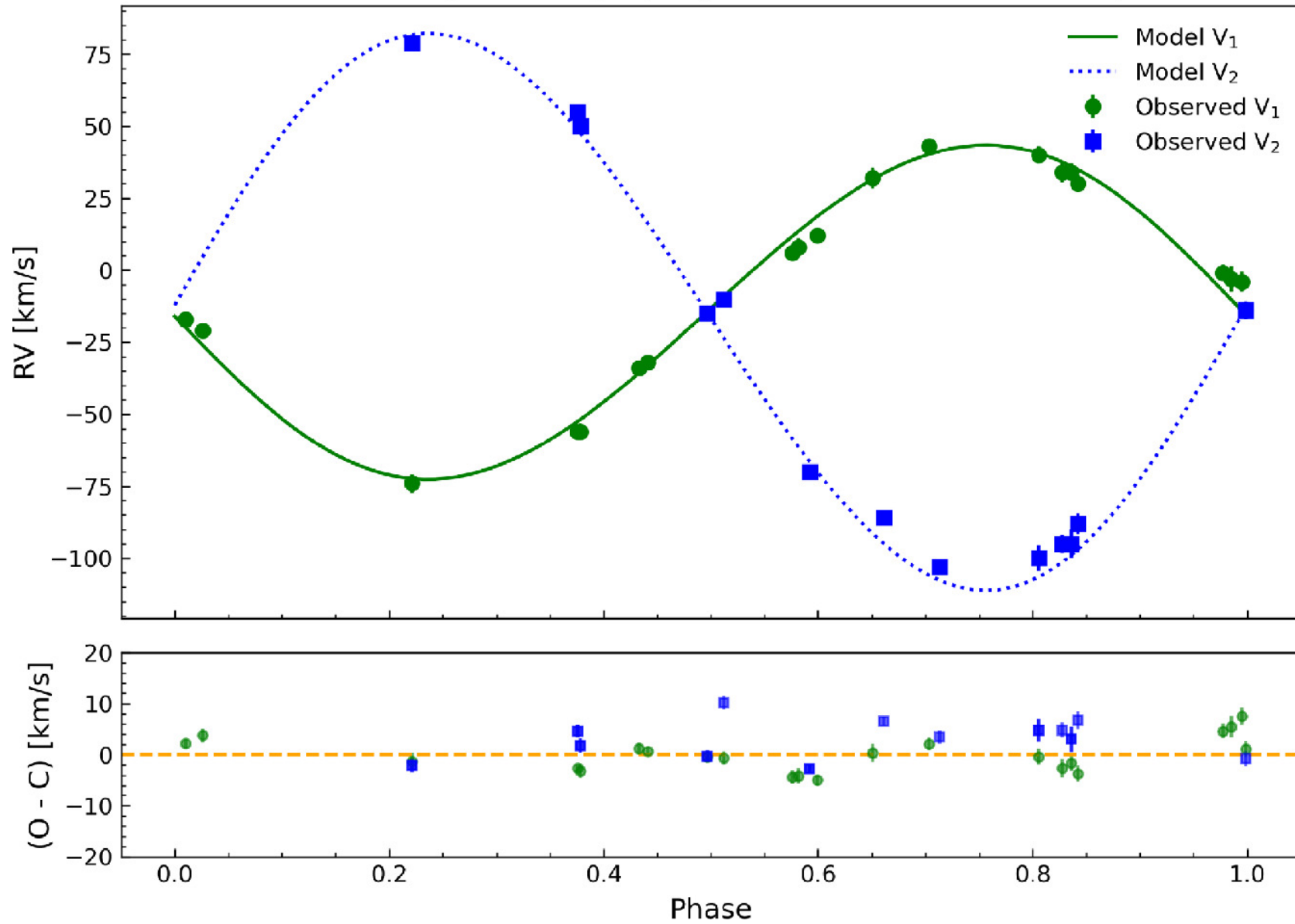
Inner binary of the triple j03 (Gaia DR3 669133613876714)
