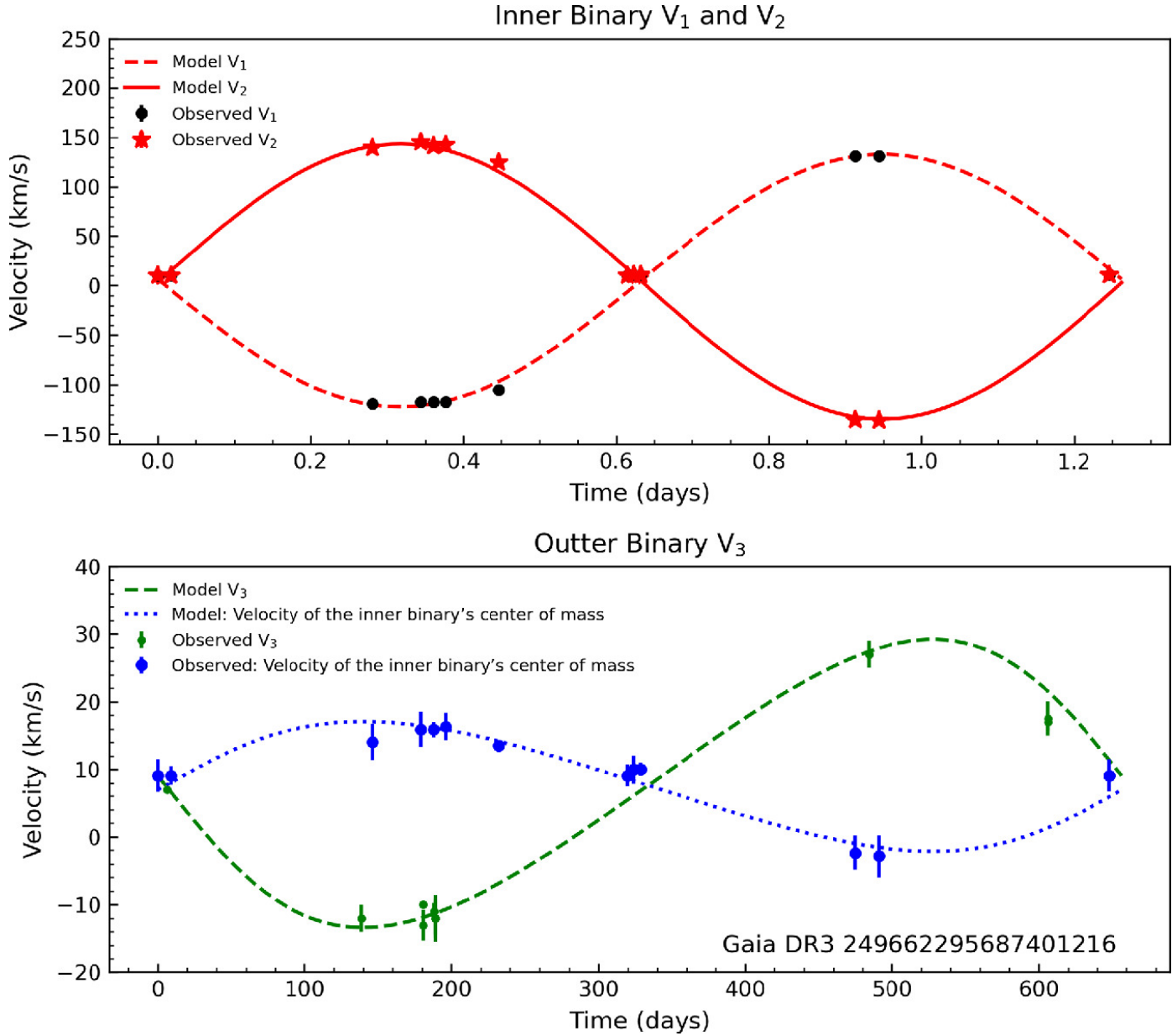
Figure 4. from Tongyu He et al 2025 Astron. J. 169 doi:10.3847/1538-3881/ad9915 https://dx.doi.org/10.3847/1538-3881/ad9915 © 2025. The Author(s). Published by the American Astronomical Society.
