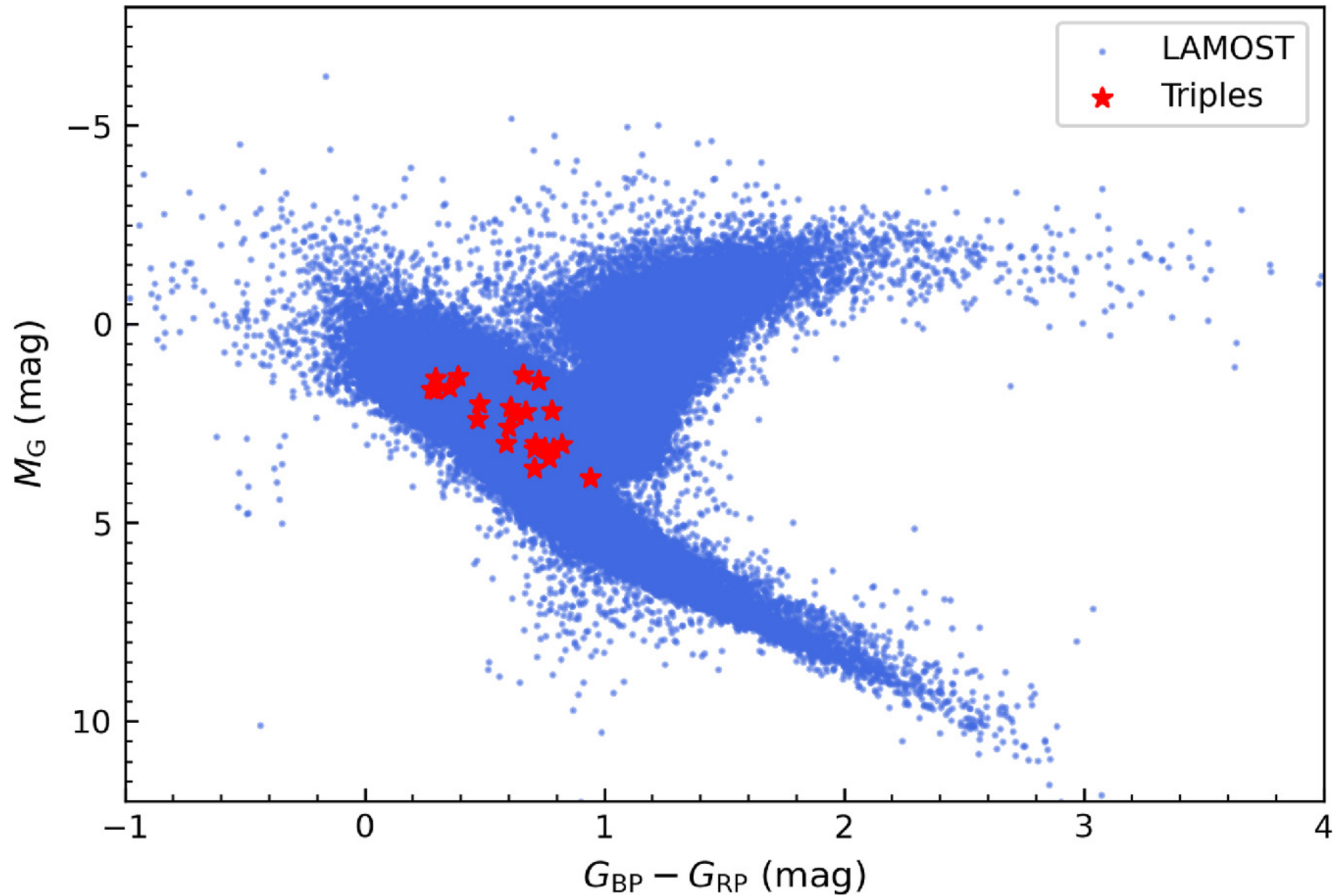
Figure 2. from Tongyu He et al 2025 Astron. J. 169 doi:10.3847/1538-3881/ad9915 https://dx.doi.org/10.3847/1538-3881/ad9915 © 2025. The Author(s). Published by the American Astronomical Society.
