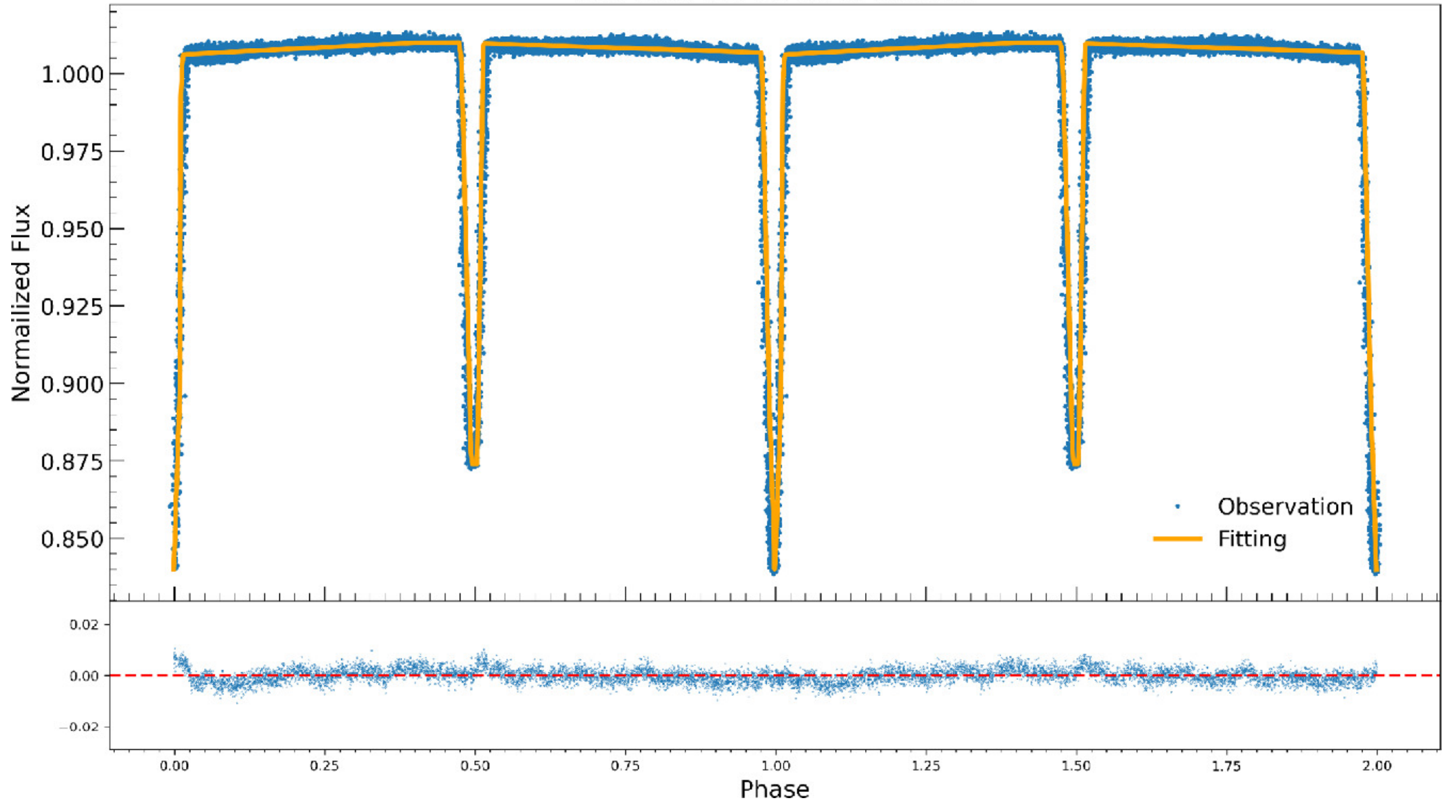
Figure 12. from Tongyu He et al 2025 Astron. J. 169 doi:10.3847/1538-3881/ad9915 https://dx.doi.org/10.3847/1538-3881/ad9915 © 2025. The Author(s). Published by the American Astronomical Society.
