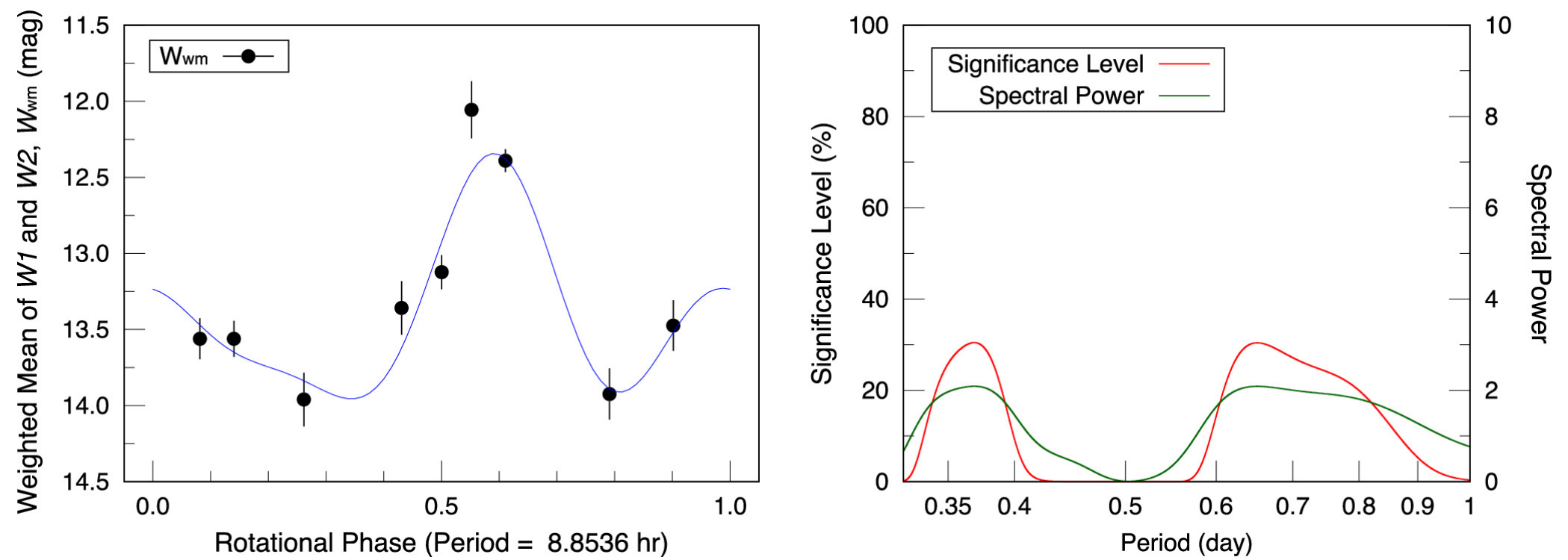
Figure 8. from Toshihiro Kasuga 2025 Astron. J. 169 doi:10.3847/1538-3881/ad95fd https://dx.doi.org/10.3847/1538-3881/ad95fd © 2025. The Author(s). Published by the American Astronomical Society.
