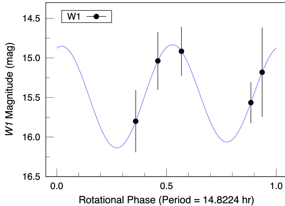
Figure 6. from Toshihiro Kasuga 2025 Astron. J. 169 doi:10.3847/1538-3881/ad95fd https://dx.doi.org/10.3847/1538-3881/ad95fd © 2025. The Author(s). Published by the American Astronomical Society.
