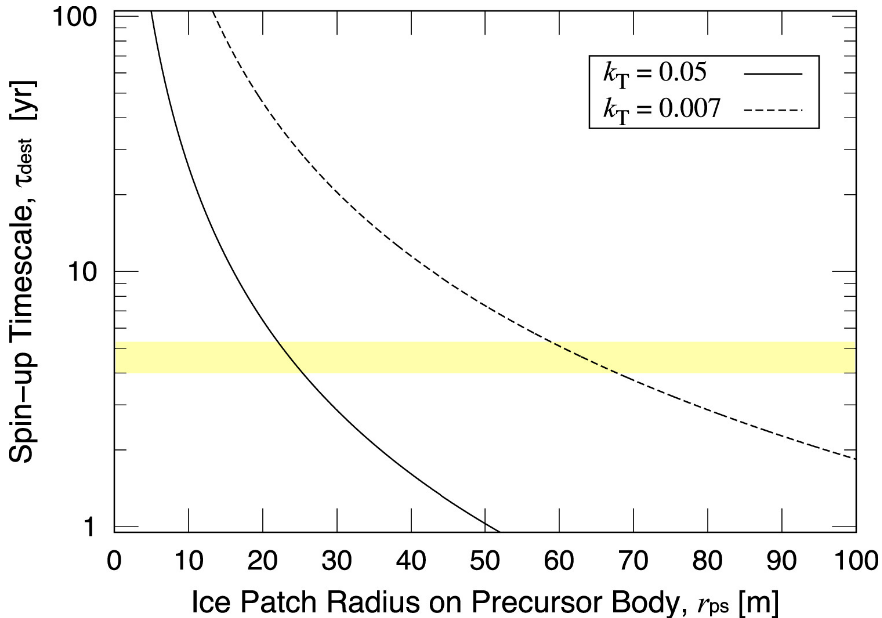
Figure 13. from Toshihiro Kasuga 2025 Astron. J. 169 doi:10.3847/1538-3881/ad95fd https://dx.doi.org/10.3847/1538-3881/ad95fd © 2025. The Author(s). Published by the American Astronomical Society.
