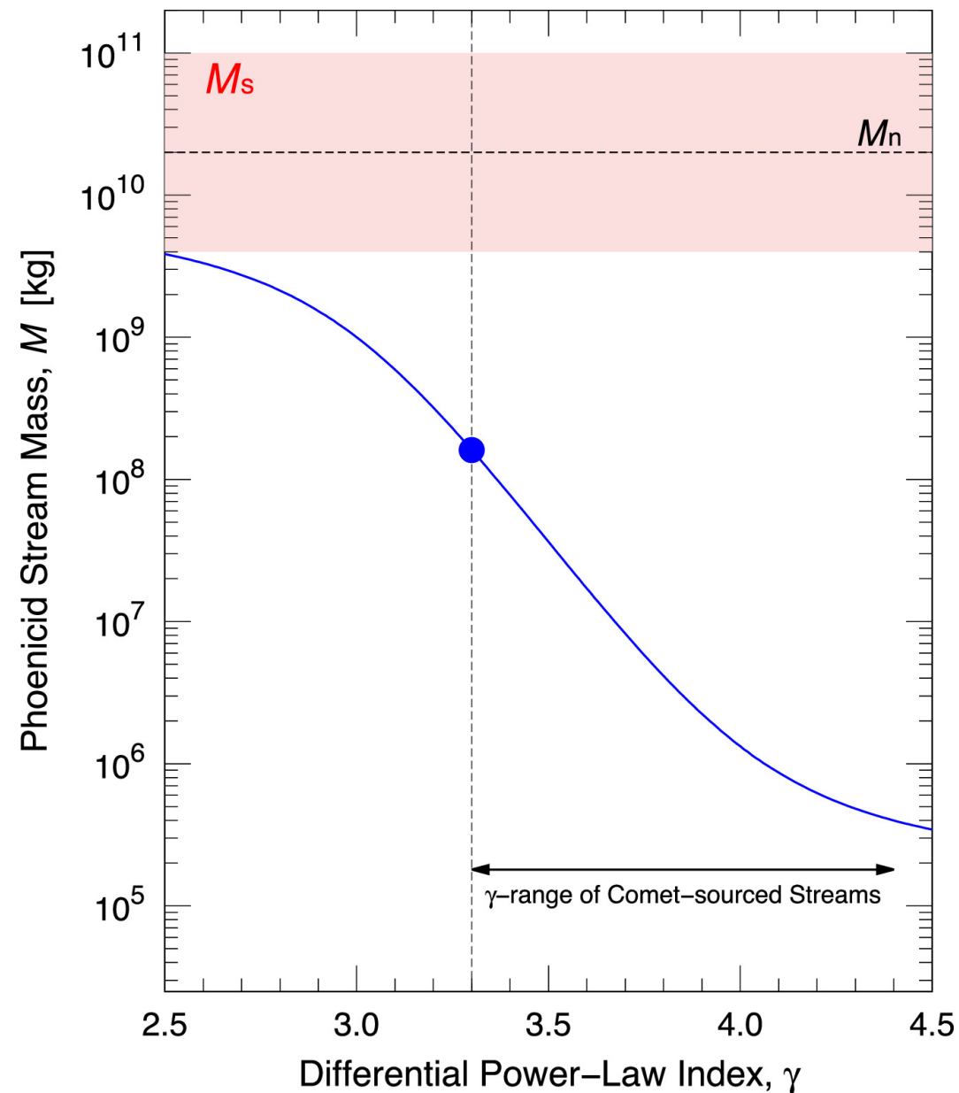
Figure 12. from Toshihiro Kasuga 2025 Astron. J. 169 doi:10.3847/1538-3881/ad95fd https://dx.doi.org/10.3847/1538-3881/ad95fd © 2025. The Author(s). Published by the American Astronomical Society.
