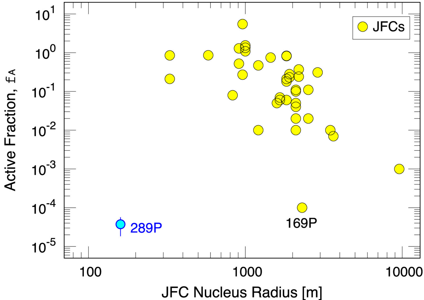
Figure 11. from Toshihiro Kasuga 2025 Astron. J. 169 doi:10.3847/1538-3881/ad95fd https://dx.doi.org/10.3847/1538-3881/ad95fd © 2025. The Author(s). Published by the American Astronomical Society.
