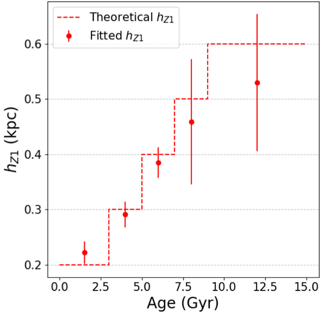
Figure 8. from Zheng Yu et al 2025 Astron. J. 169 doi:10.3847/1538-3881/ad9582 https://dx.doi.org/10.3847/1538-3881/ad9582 © 2025. The Author(s). Published by the American Astronomical Society.
