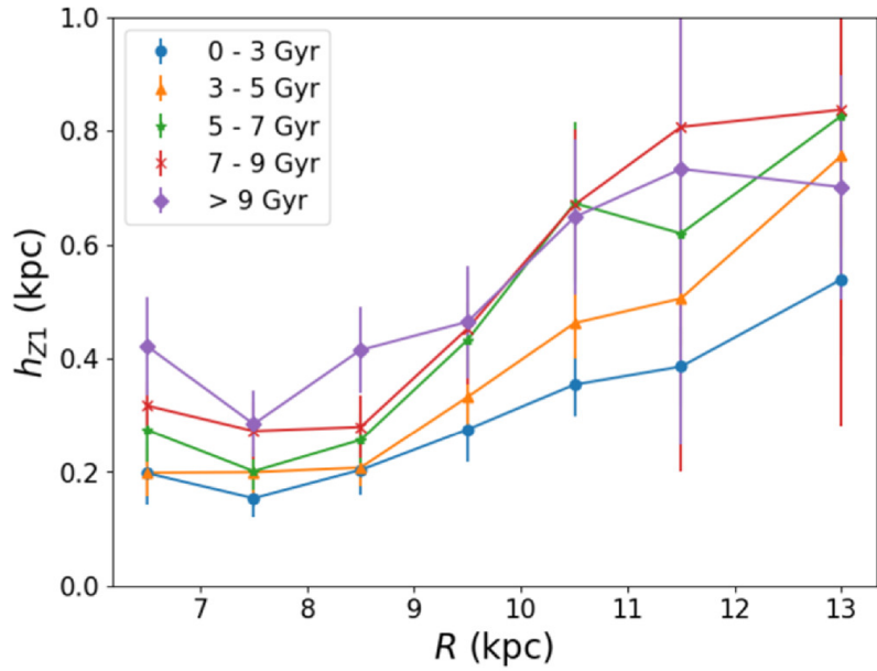
Figure 5. from Zheng Yu et al 2025 Astron. J. 169 doi:10.3847/1538-3881/ad9582 https://dx.doi.org/10.3847/1538-3881/ad9582 © 2025. The Author(s). Published by the American Astronomical Society.
