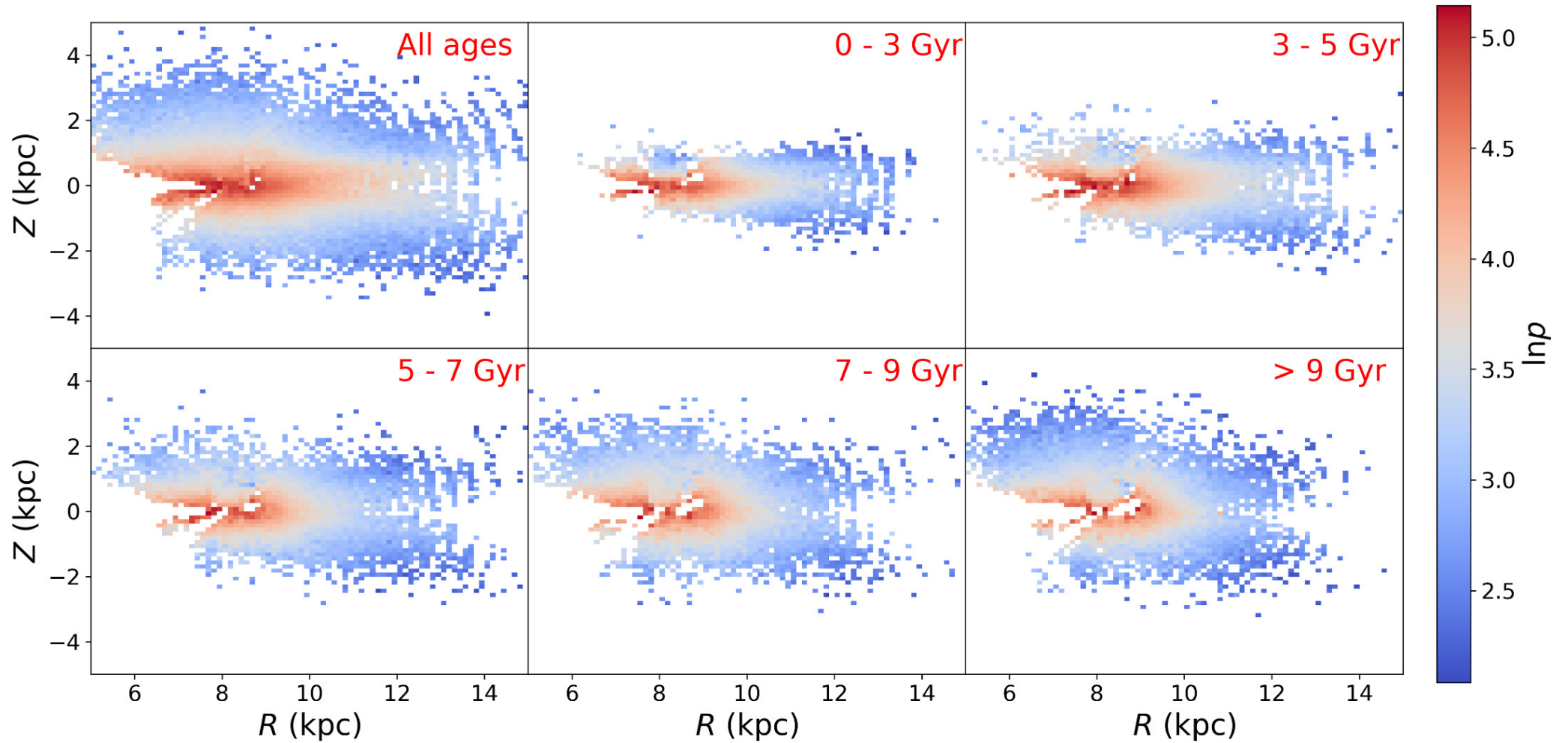
Figure 3. from Zheng Yu et al 2025 Astron. J. 169 doi:10.3847/1538-3881/ad9582 https://dx.doi.org/10.3847/1538-3881/ad9582 © 2025. The Author(s). Published by the American Astronomical Society.
