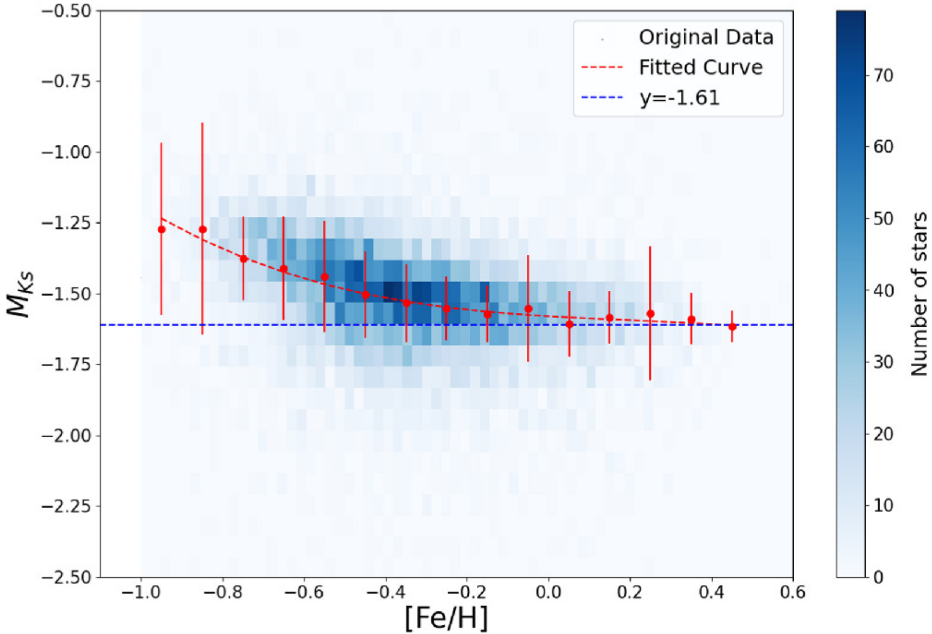
Figure 1. from Zheng Yu et al 2025 Astron. J. 169 doi:10.3847/1538-3881/ad9582 https://dx.doi.org/10.3847/1538-3881/ad9582 © 2025. The Author(s). Published by the American Astronomical Society.
