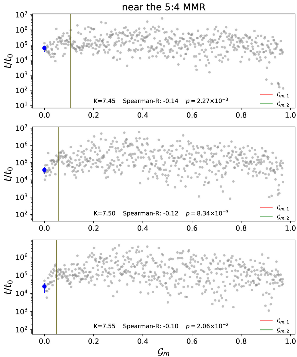
Figure 5. from Dong-Hong Wu et al 2025 Astron. J. 169 doi:10.3847/1538-3881/ad9388 https://dx.doi.org/10.3847/1538-3881/ad9388 © 2024. The Author(s). Published by the American Astronomical Society.
