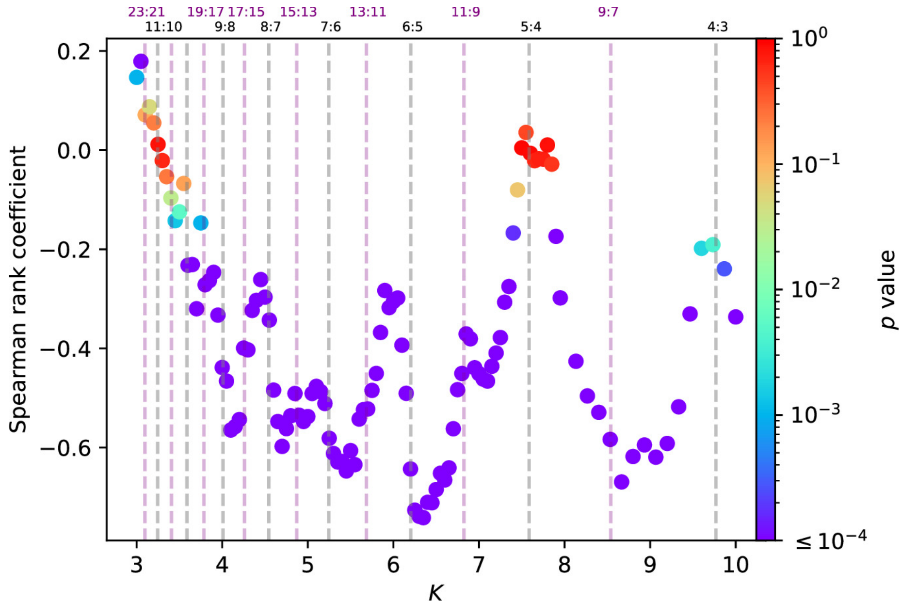
Figure 2. from Dong-Hong Wu et al 2025 Astron. J. 169 doi:10.3847/1538-3881/ad9388 https://dx.doi.org/10.3847/1538-3881/ad9388 © 2024. The Author(s). Published by the American Astronomical Society.
