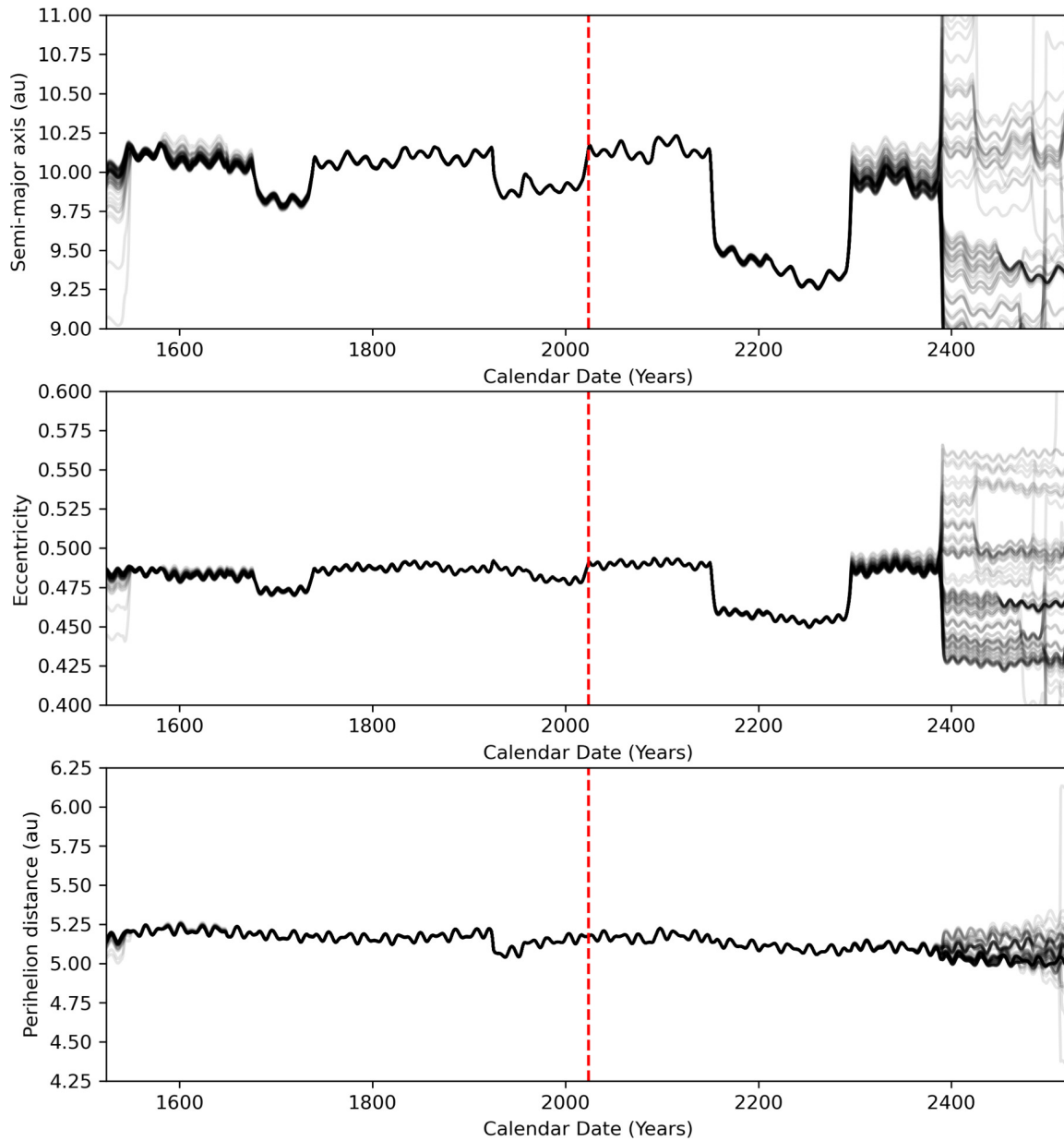
Figure 9. from Matthew M. Dobson et al 2024 Astron. J. 168 doi:10.3847/1538-3881/ad8a5f https://dx.doi.org/10.3847/1538-3881/ad8a5f © 2024. The Author(s). Published by the American Astronomical Society.
