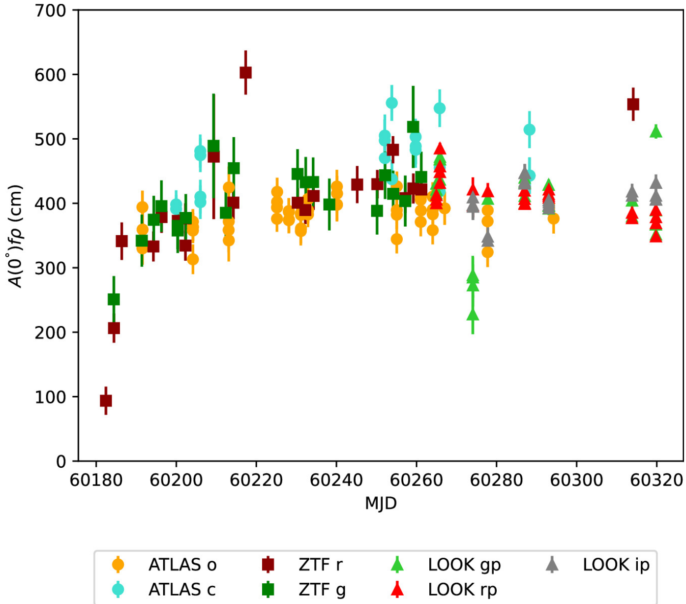
Figure 8. from Matthew M. Dobson et al 2024 Astron. J. 168 doi:10.3847/1538-3881/ad8a5f https://dx.doi.org/10.3847/1538-3881/ad8a5f © 2024. The Author(s). Published by the American Astronomical Society.
