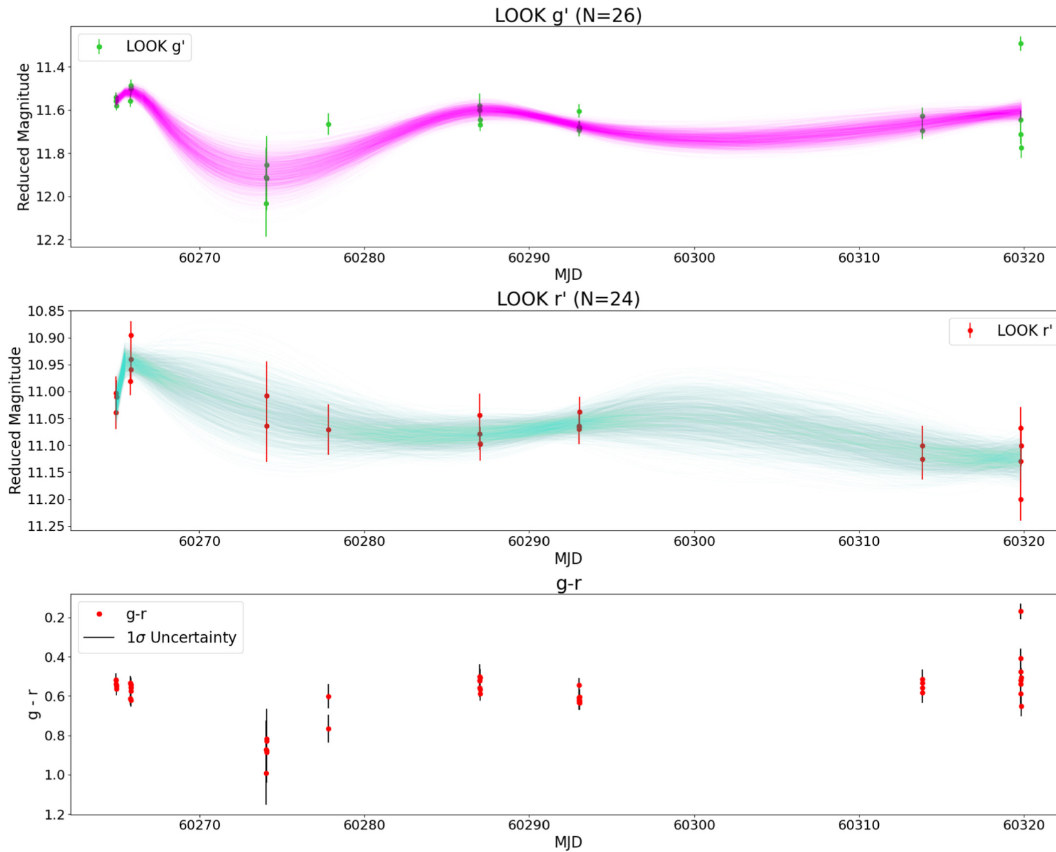
Figure 5. from Matthew M. Dobson et al 2024 Astron. J. 168 doi:10.3847/1538-3881/ad8a5f https://dx.doi.org/10.3847/1538-3881/ad8a5f © 2024. The Author(s). Published by the American Astronomical Society.
