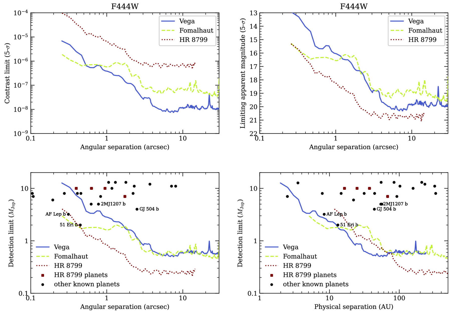
Figure 9. from Charles Beichman et al 2025 Astron. J. 169 doi:10.3847/1538-3881/ad890d https://dx.doi.org/10.3847/1538-3881/ad890d © 2024. The Author(s). Published by the American Astronomical Society.
