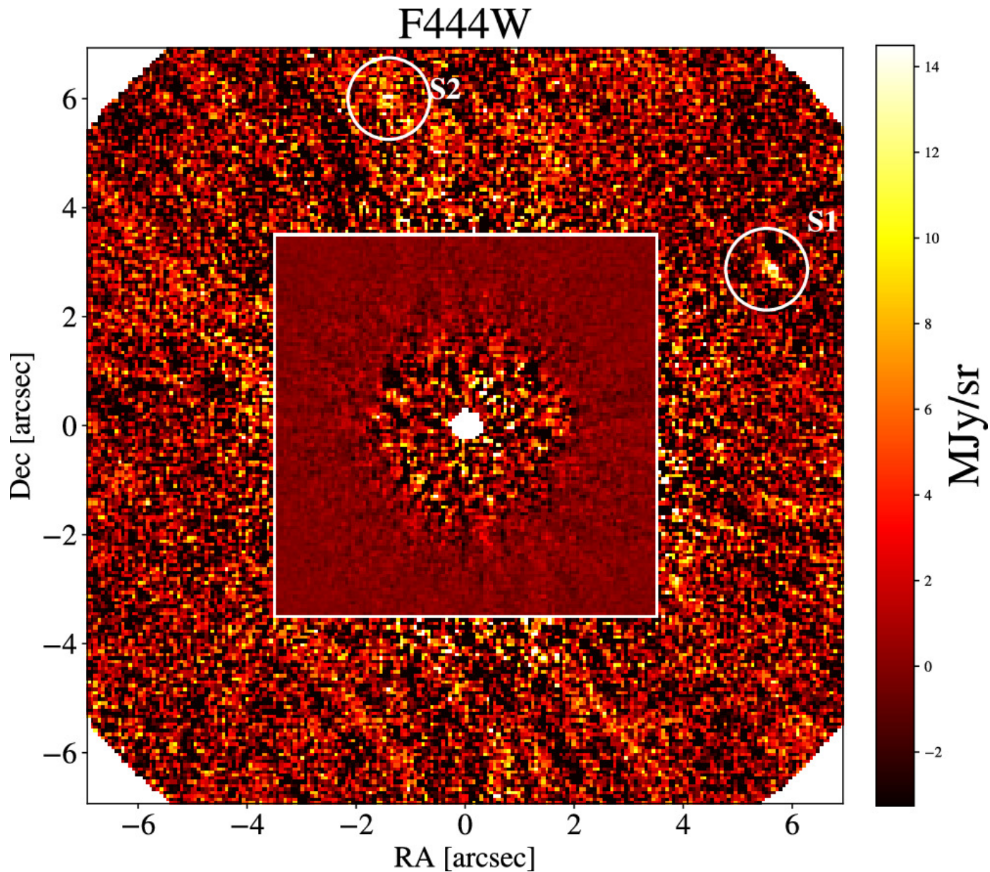
Figure 4. from Charles Beichman et al 2025 Astron. J. 169 doi:10.3847/1538-3881/ad890d https://dx.doi.org/10.3847/1538-3881/ad890d © 2024. The Author(s). Published by the American Astronomical Society.
