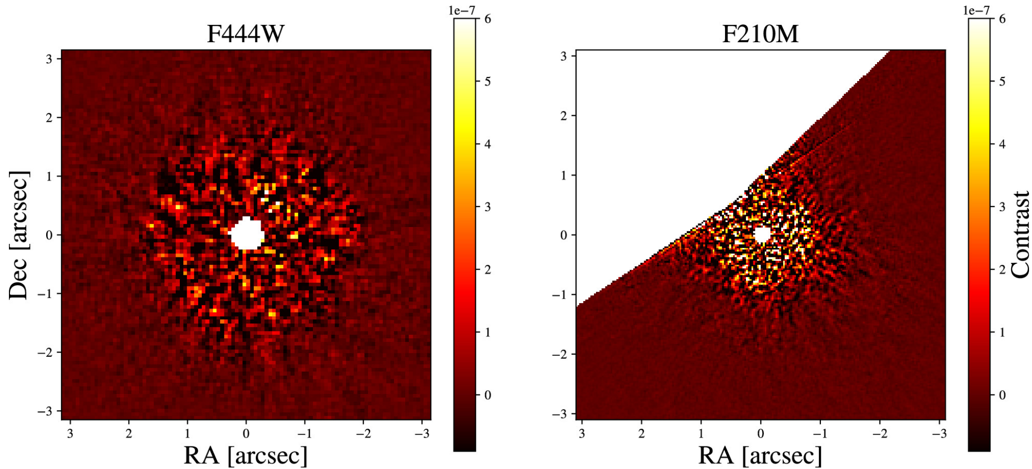
Figure 3. from Charles Beichman et al 2025 Astron. J. 169 doi:10.3847/1538-3881/ad890d https://dx.doi.org/10.3847/1538-3881/ad890d © 2024. The Author(s). Published by the American Astronomical Society.
