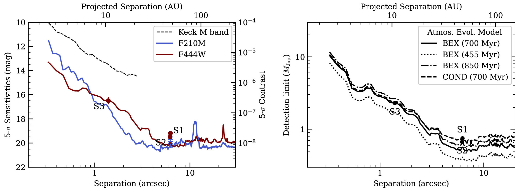
Figure 2. from Charles Beichman et al 2025 Astron. J. 169 doi:10.3847/1538-3881/ad890d https://dx.doi.org/10.3847/1538-3881/ad890d © 2024. The Author(s). Published by the American Astronomical Society.
