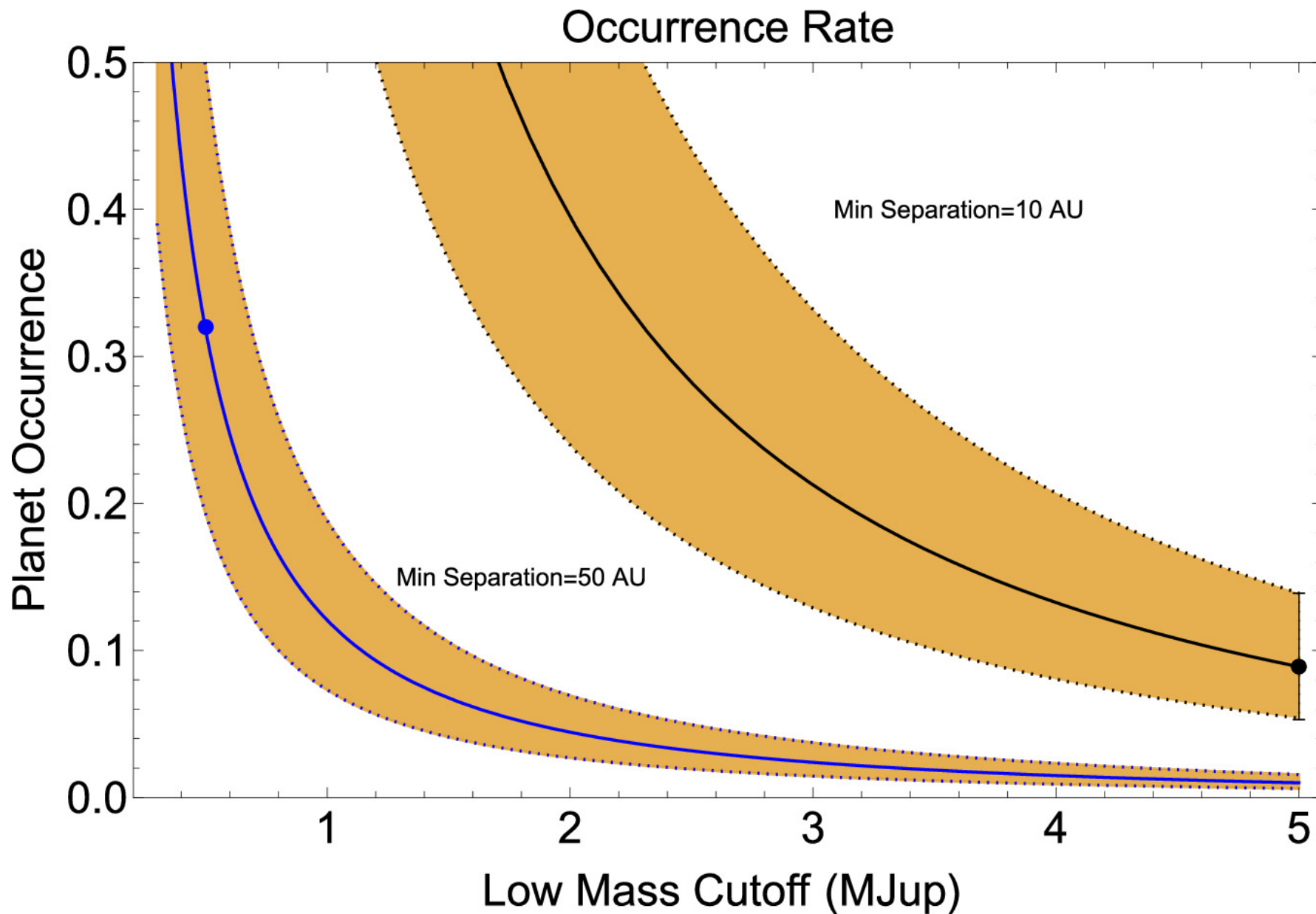
Figure 10. from Charles Beichman et al 2025 Astron. J. 169 doi:10.3847/1538-3881/ad890d https://dx.doi.org/10.3847/1538-3881/ad890d © 2024. The Author(s). Published by the American Astronomical Society.
