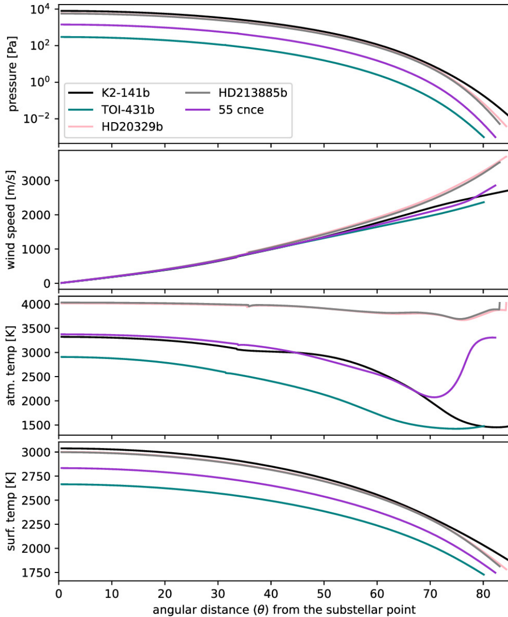
Figure 2. from T. Giang Nguyen et al 2024 Astron. J. 168 doi:10.3847/1538-3881/ad85e0 https://dx.doi.org/10.3847/1538-3881/ad85e0 © 2024. The Author(s). Published by the American Astronomical Society.
