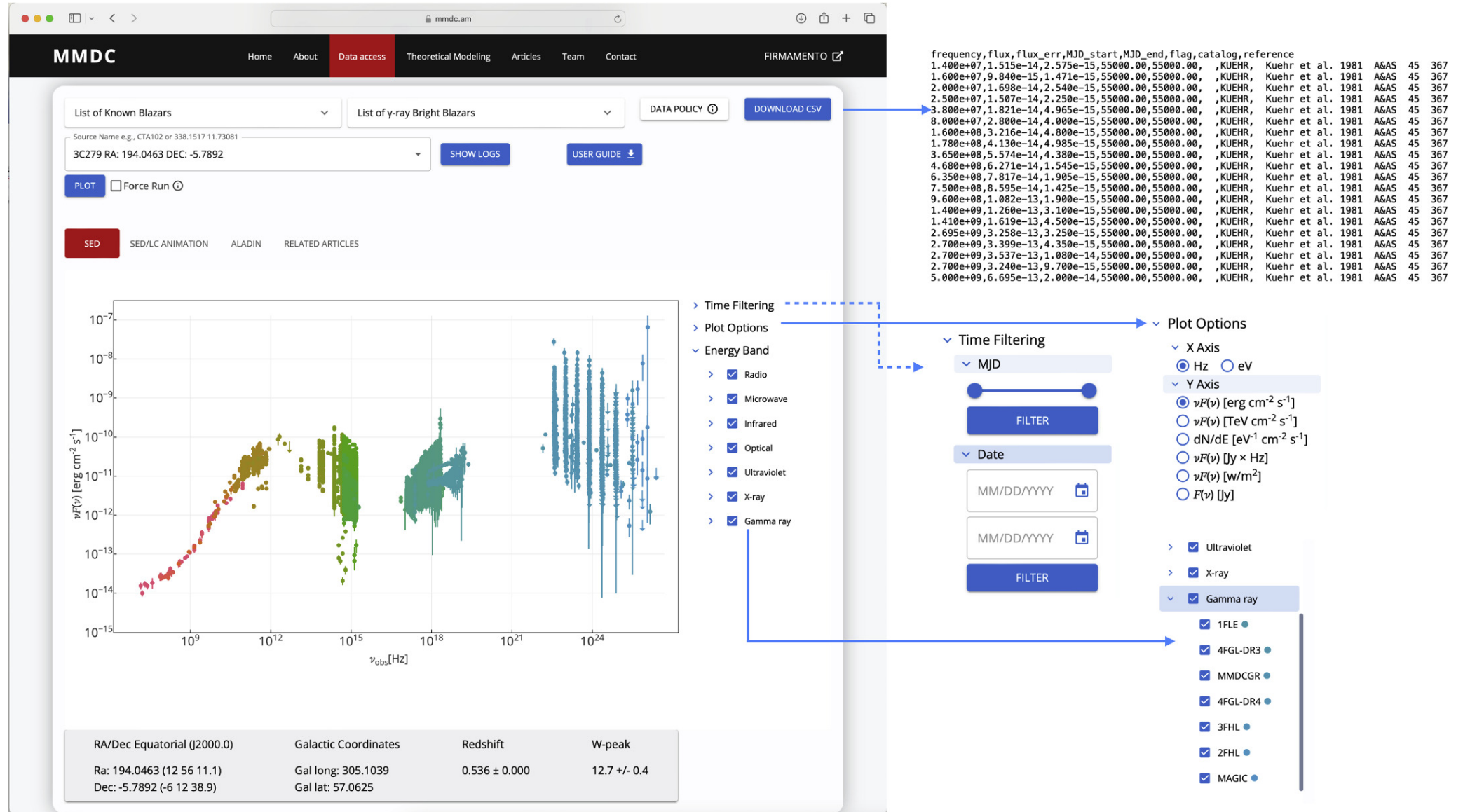
Figure 5. from N. Sahakyan et al 2024 Astron. J. 168 doi:10.3847/1538-3881/ad8231 https://dx.doi.org/10.3847/1538-3881/ad8231 © 2024. The Author(s). Published by the American Astronomical Society.
